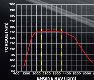
Max. Torque of 152Nm (Flat Torque Curve) at a low 2,400 - 4,000rpm
